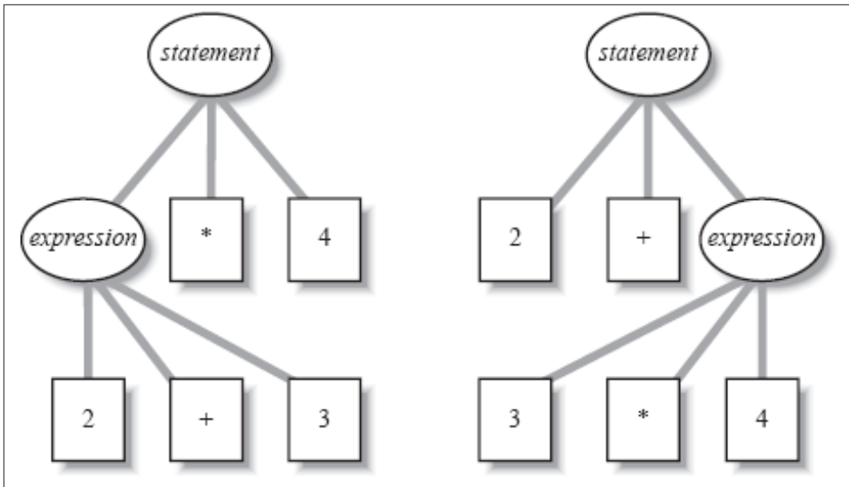
Figure 3-3. Ambiguous input 2+3*4
