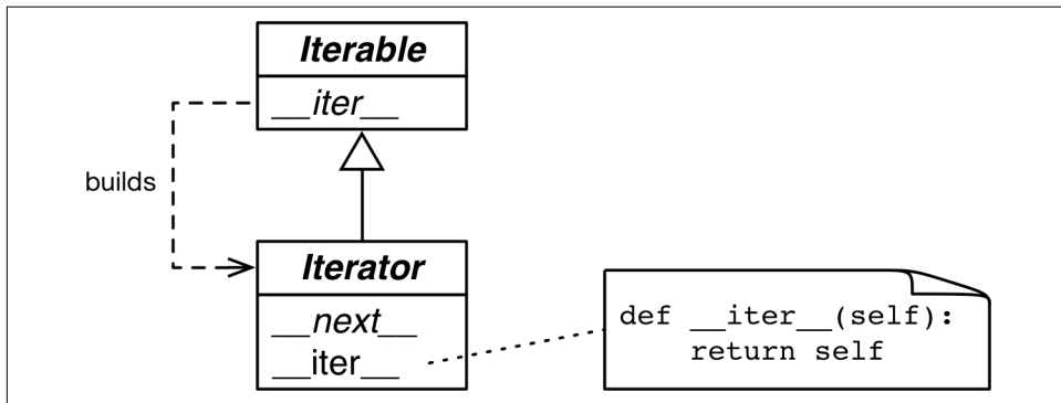
Figure 14-1. The Iterable and Iterator ABCs. Methods in italic are abstract. A concrete Iterable . __iter__ should return a new Iterator instance. A concrete Iterator must implement __next__ . The Iterator . __iter__ method just returns the instance itself.
