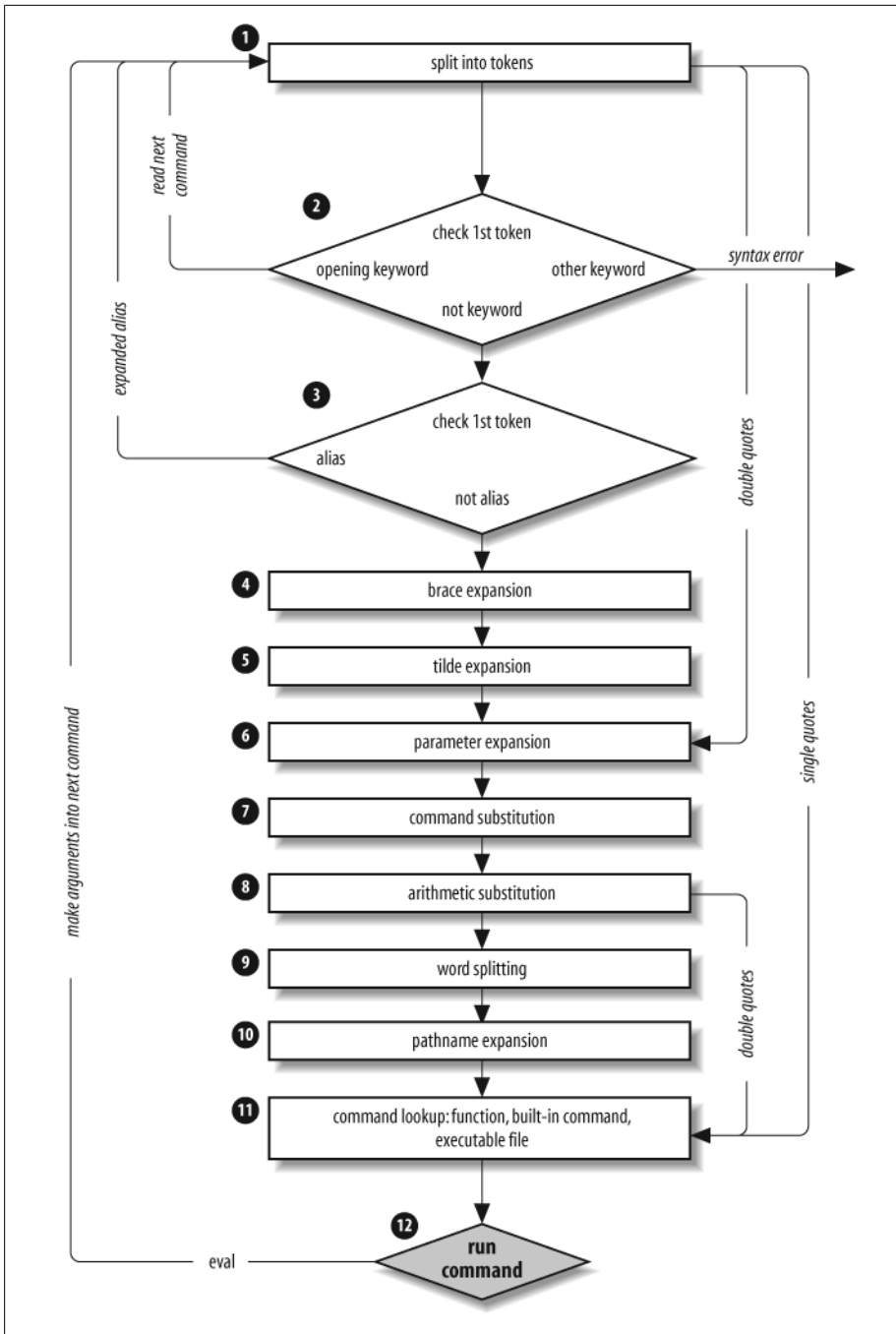
Figure C-1. Steps in command-line processing
