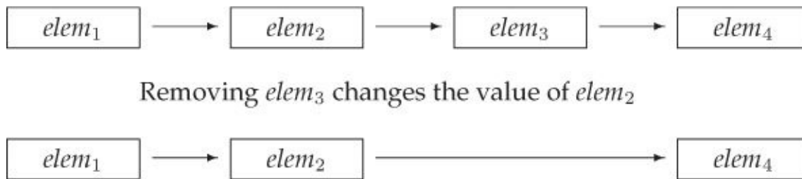
Figure 9.1. forward_list Specialized Operations
