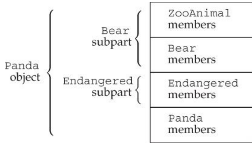
Figure 18.2. Conceptual Structure of a Panda Object
