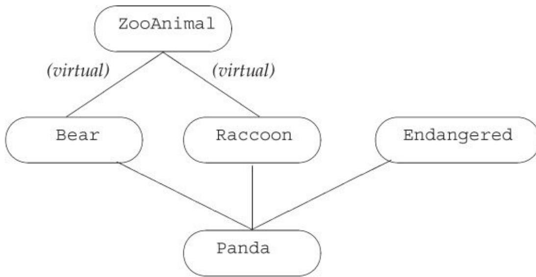
Figure 18.3. Virtual Inheritance Panda Hierarchy
