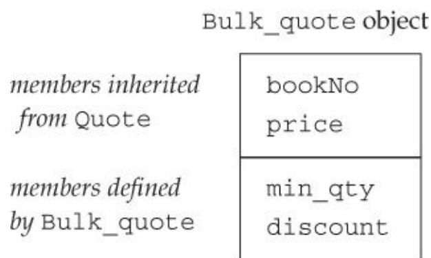
Figure 15.1. Conceptual Structure of a Bulk_quote Object
