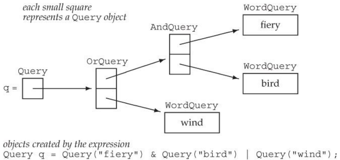
Figure 15.3. Objects Created by Query Expressions
