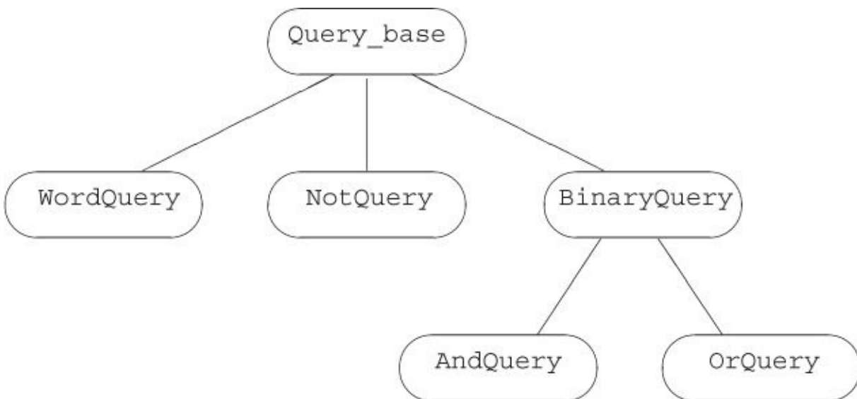
Figure 15.2. Query_base Inheritance Hierarchy
