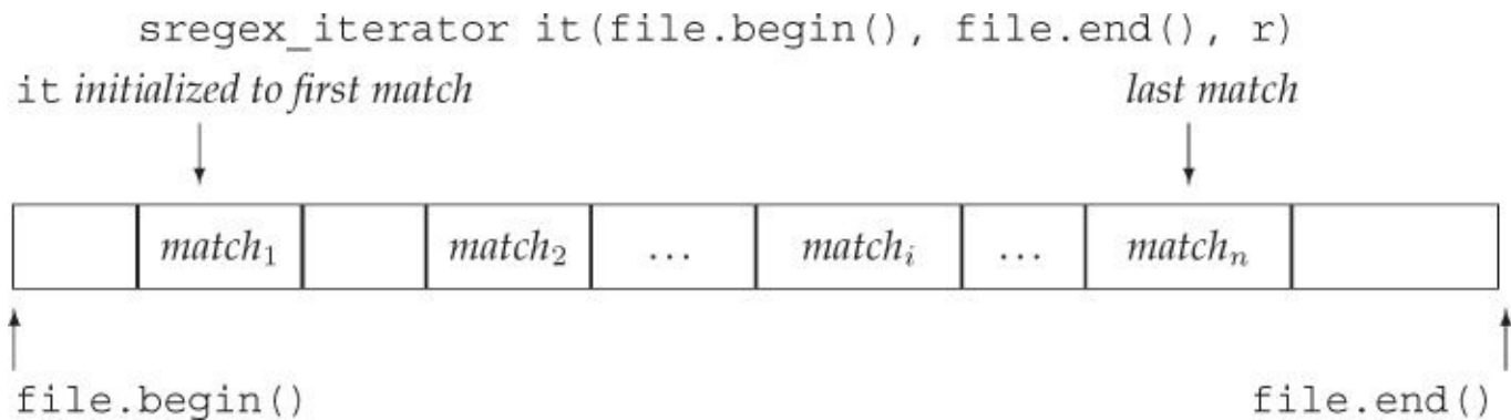
Figure 17.1. Using an sregex_iterator
