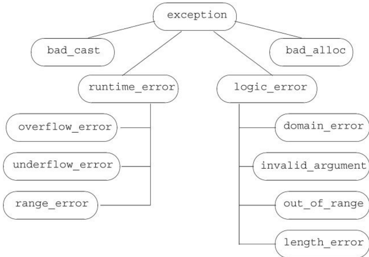
Figure 18.1. Standard exception Class Hierarchy
