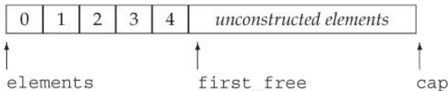
Figure 13.2. StrVec Memory Allocation Strategy
