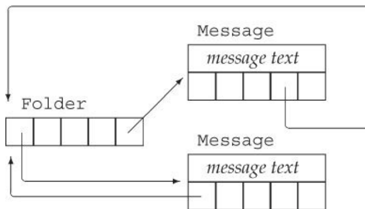
Figure 13.1. Message and Folder Class Design
