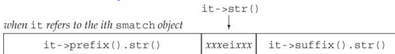
Figure 17.2. The smatch Object Representing a Particular Match
