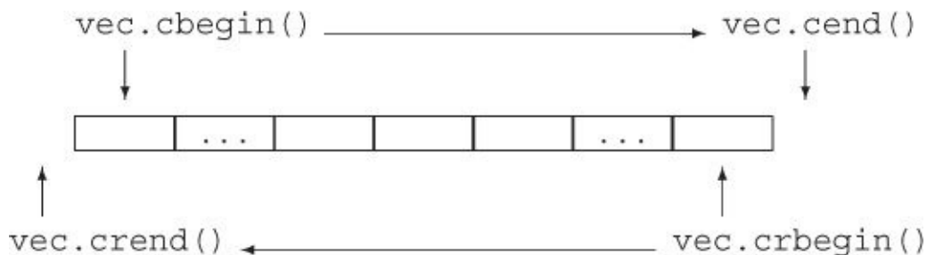
Figure 10.1. Comparing begin/cend and rbegin/crend Iterators
